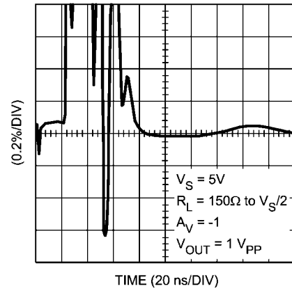
Output Settling
