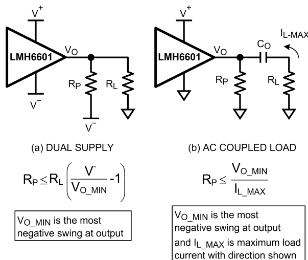
FIGURE 2. Output Pull-Down Value for Dual Supply & AC Coupling
