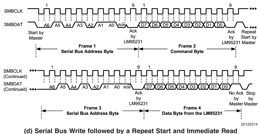
FIGURE 2. SMBus Timing Diagrams for Access of Data
