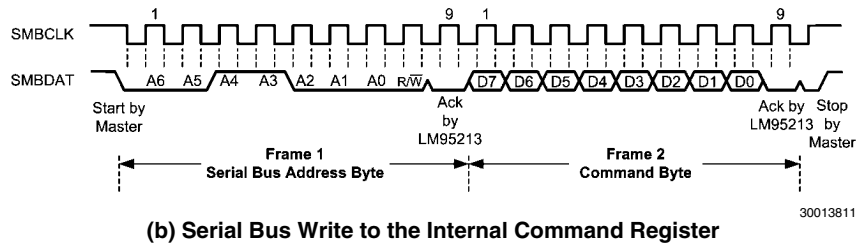
(b) Serial Bus Write to the Internal Command Register
