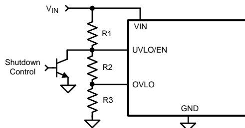
Figure 16. Shutdown Control
