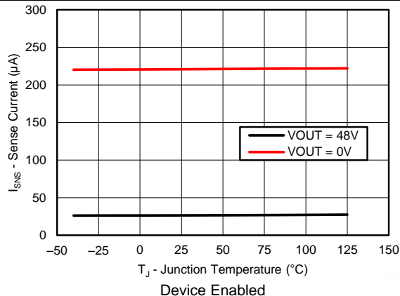
Figure 3. Sense Current vs V_{OUT} and T_J
