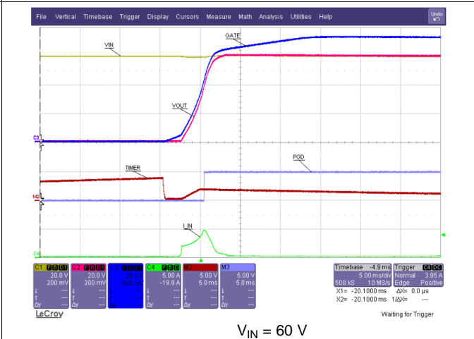
Figure 31. Start-Up
