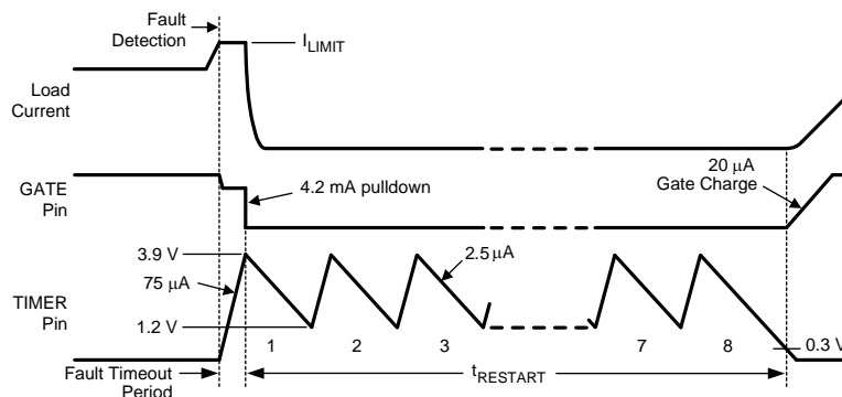
Figure 15. Restart Sequence
