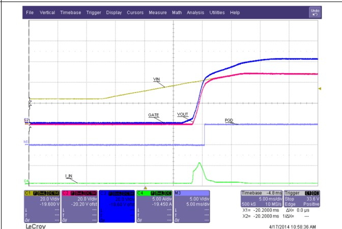
Figure 31. Start-Up
