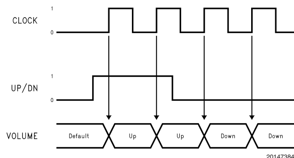
FIGURE 2. Timing Diagram
