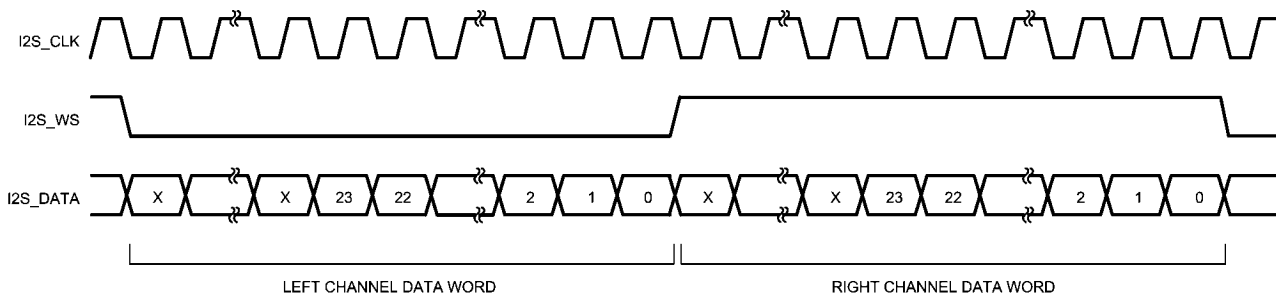
FIGURE 7. I 2 S Right Justified Input Format
