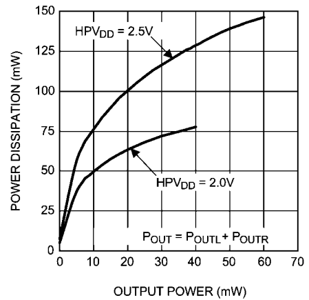
Power Dissipation vs Output Power R_L = 32\Omega , f = 1\text{kHz} , Headphone Mode
