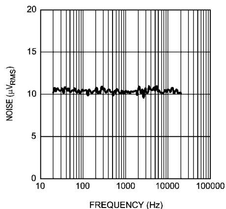
Output Noise vs Frequency V_{DD} = 2.5\text{V} , R_L = 32\Omega DAC Input, Internal Reference, Headphone Mode
