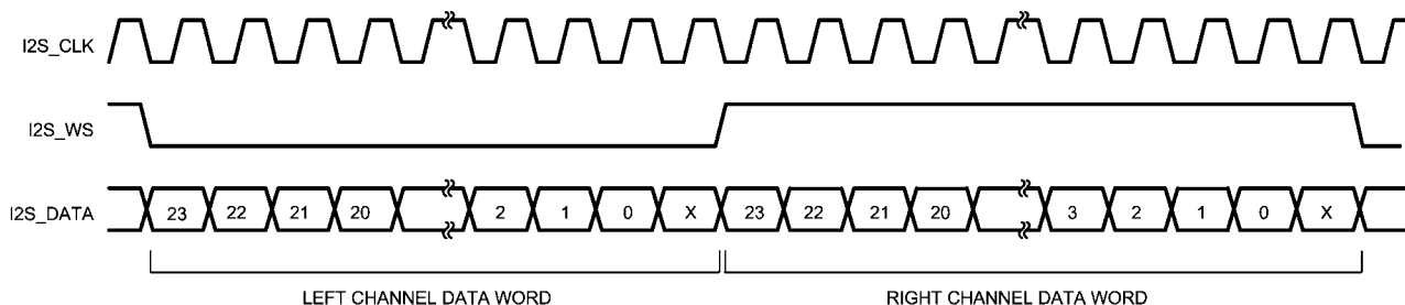
FIGURE 6. I 2 S Left Justified Input Format
