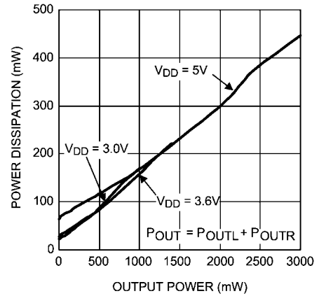
Power Dissipation vs Output Power R_L = 8\Omega , f = 1\text{kHz} , Speaker Mode
