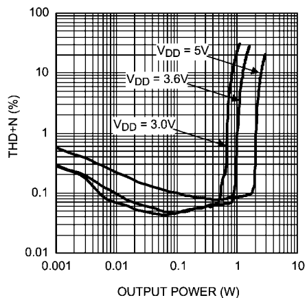
THD+N vs Output Power A_V = 12\text{dB} , R_L = 4\Omega , f = 1\text{kHz} DAC Input, Internal Reference, Speaker Mode
