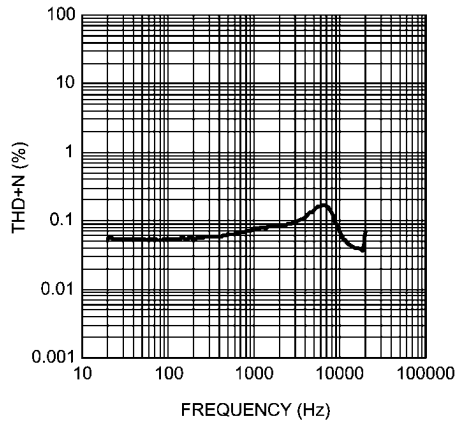
THD+N vs Frequency V_{DD} = 5.0V , P_{OUT} = 750mW , R_L = 4\Omega DAC Input, Internal Reference, Speaker Mode
