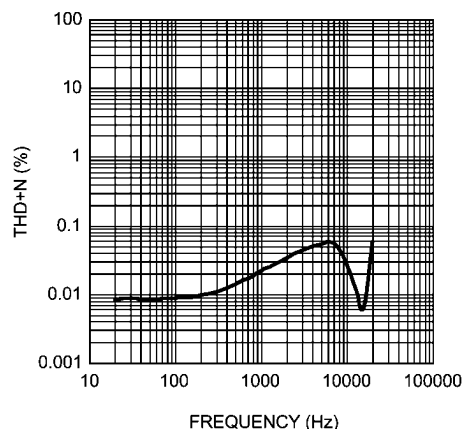
THD+N vs Frequency HPV_{DD} = 2.0V , P_{OUT} = 10mW , R_L = 16\Omega DAC Input, Internal Reference, Headphone Mode
