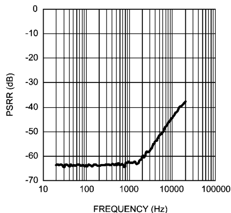
PSRR vs Frequency V_{DD} = 3.6V , V_{RIPPLE} = 200mV_{P-P} , R_L = 8\Omega DAC Input, External Reference, Speaker Mode
