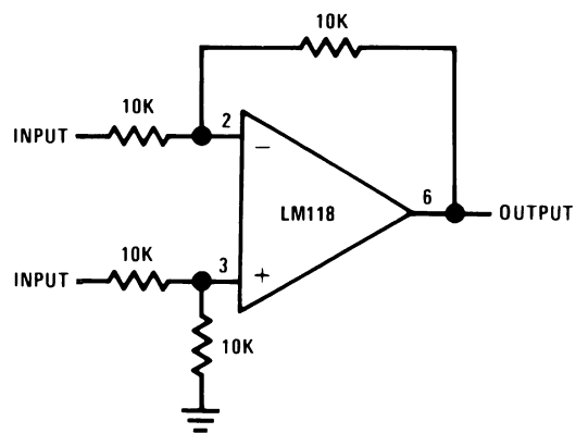
Differential Amplifier
