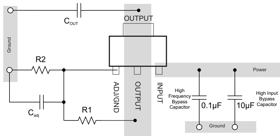
Figure 11. Layout Diagram
