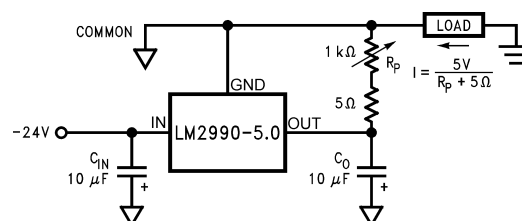
Figure 25. Adjustable Current Sink
