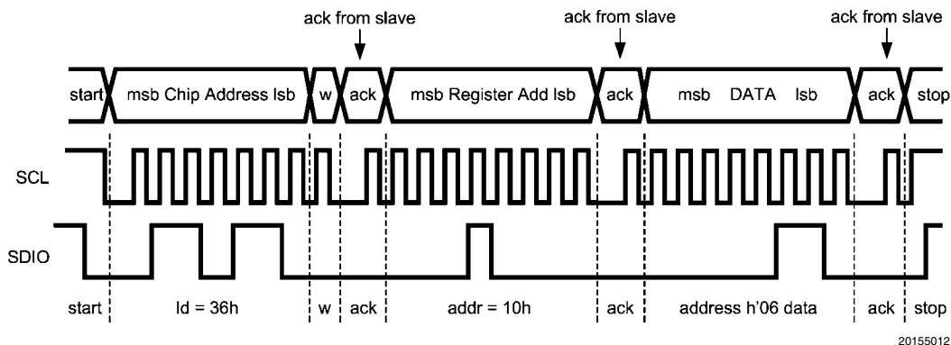
FIGURE 3. Write Cycle
