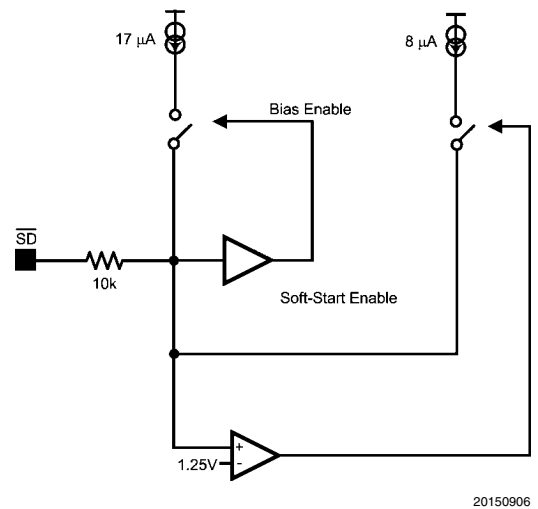
FIGURE 8. \overline{\text{SD}} Pin Logic
