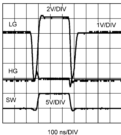
Switch Waveforms
