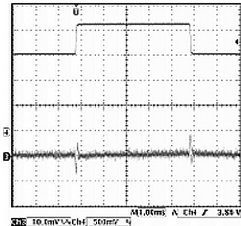
Line Transient (LDO1) 3.6 - 4.2V_{IN} , 2.5V_{OUT} , 100 mA load
