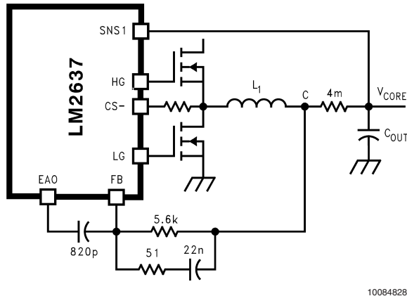
FIGURE 10. Dynamic Voltage Positioning by Using a Stand-Alone Resistor
