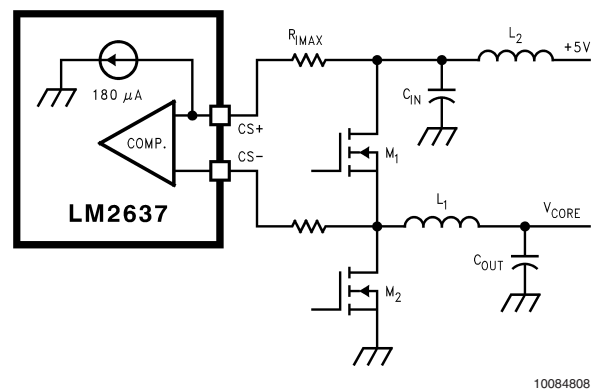
FIGURE 4. Current Limit via High-Side FET V_{DS} Sensing
