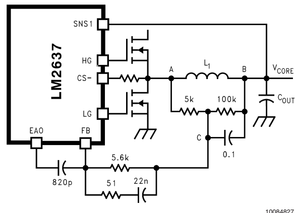
FIGURE 9. Dynamic Voltage Positioning by Utilizing Output Inductor DC Resistance
