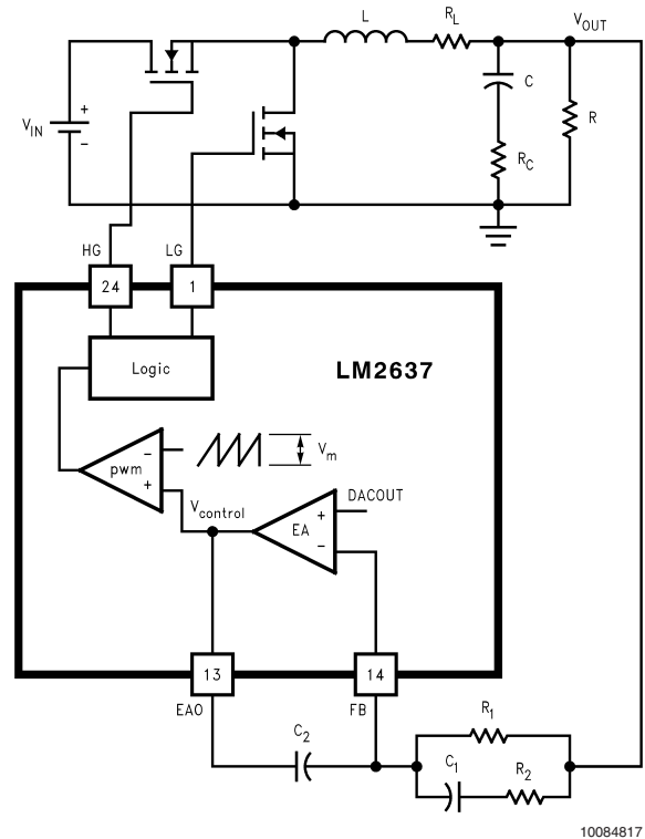
FIGURE 6. Buck Converter from a Control Viewpoint
