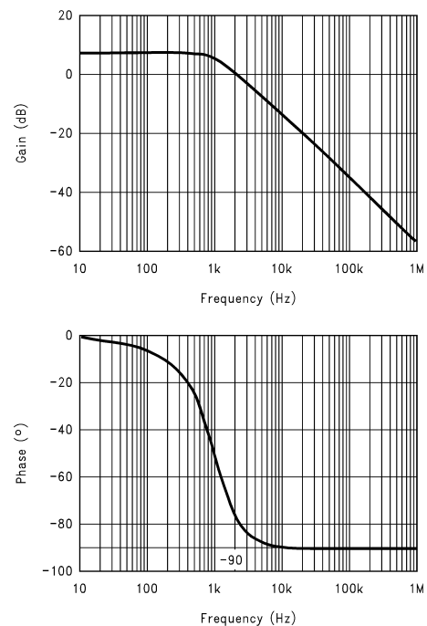
FIGURE 7. Control-to-Output Bode Plots
