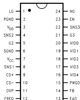
24-Lead SOIC
