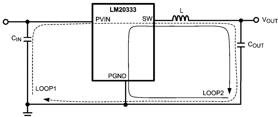
FIGURE 13. Schematic of LM20333 Highlighting Layout Sensitive Nodes
