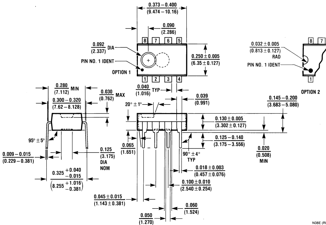
Molder Dual-In-Line Package Order Number LF353N NS Package Number N08E
