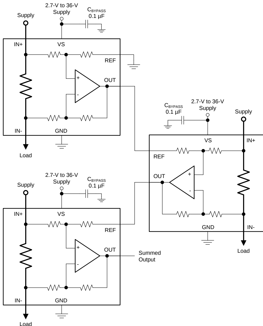
Figure 37. Daisy-Chain Configuration
