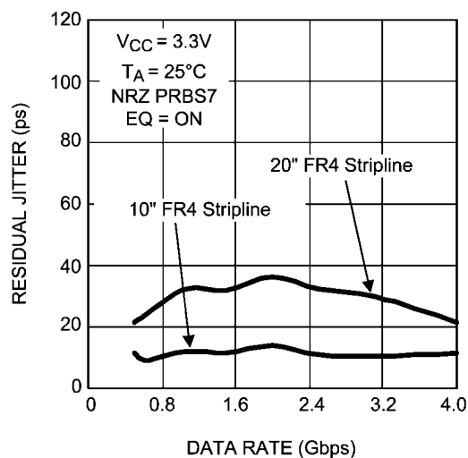
30008052 Residual Jitter as a Function of Data Rate, FR4 Stripline Length and EQ Level
