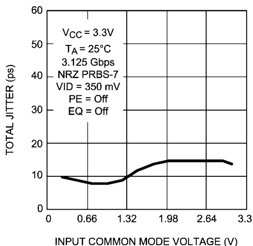
30008058 Total Jitter as a Function of Input Common Mode Voltage
