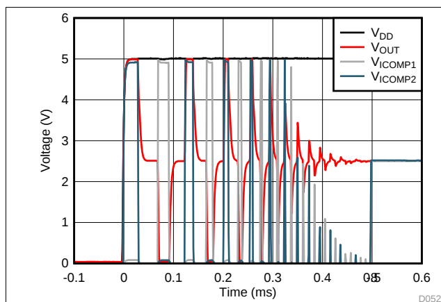
Figure 61. Demagnetization Sequence
