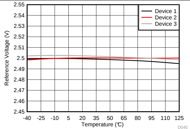
Figure 44. Reference Voltage vs Temperature
