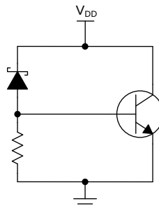
Figure 64. Additonal Supply Clamp for the DRV421
