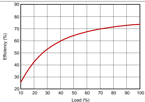
Figure 26. Efficiency vs Load
