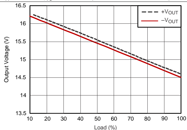
Figure 25. Load Regulation
