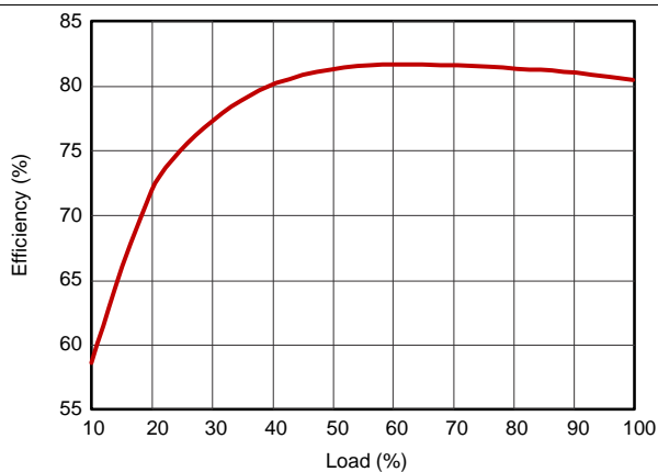
DCP010505B Efficiency
