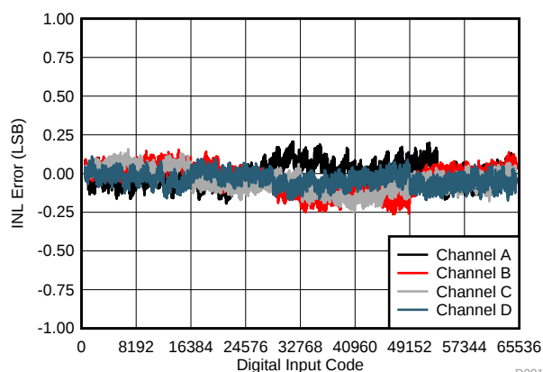
Linearity Error vs Digital Input Code
