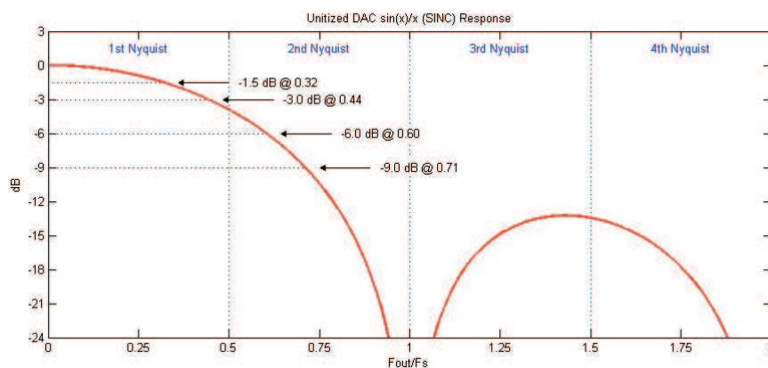
Figure 40. Unitized DAC \sin(x)/x (SINC) Response
