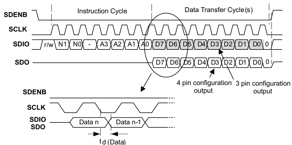
Figure 17. Serial Interface Read Timing Diagram
