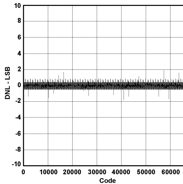
Figure 2. Differential Nonlinearity
