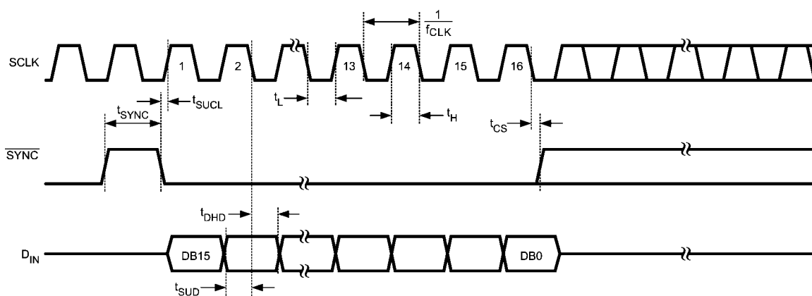
FIGURE 2. DAC101S101 Timing
