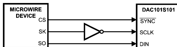
FIGURE 8. Microwire Interface
