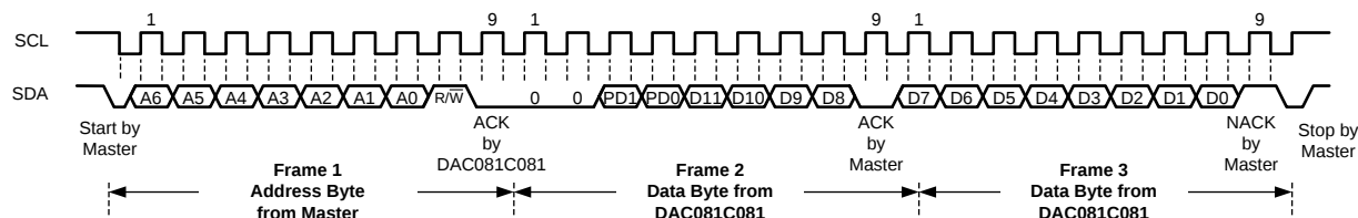
Figure 24. Typical Read from the DAC Register
