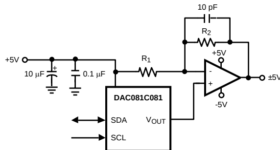
Figure 31. Bipolar Operation
