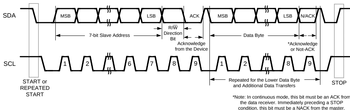
Figure 21. Basic Operation.
