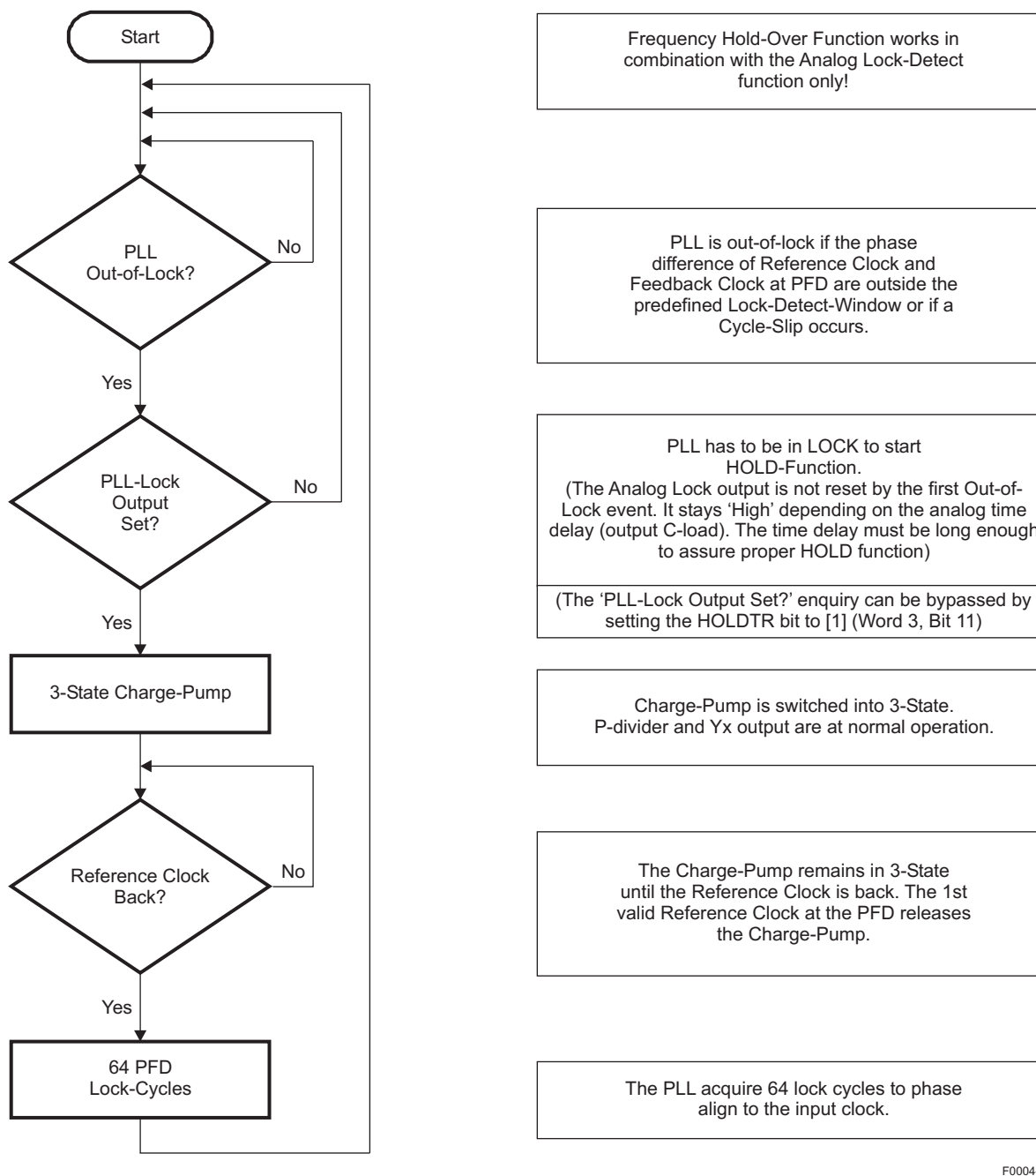
Figure 22. Frequency HOLD-Over Function
