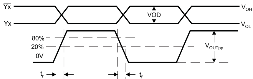
Figure 9. LVPECL Differential Output Voltage and Rise/Fall Time
