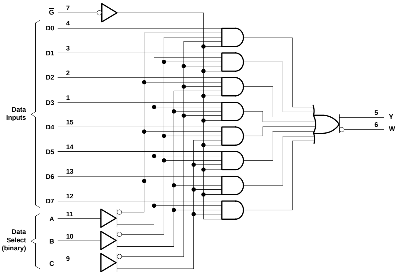
logic diagram (positive logic)
