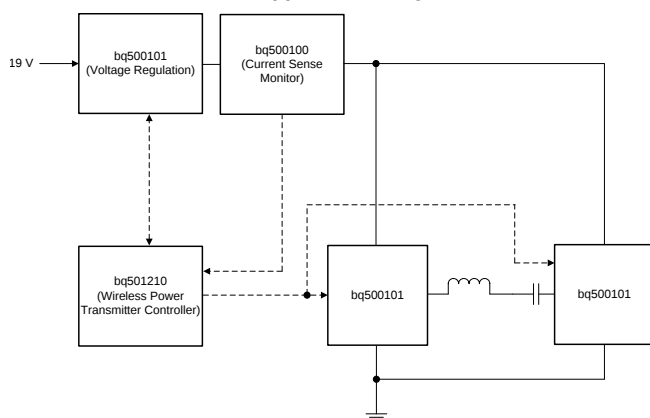
Application Diagram
