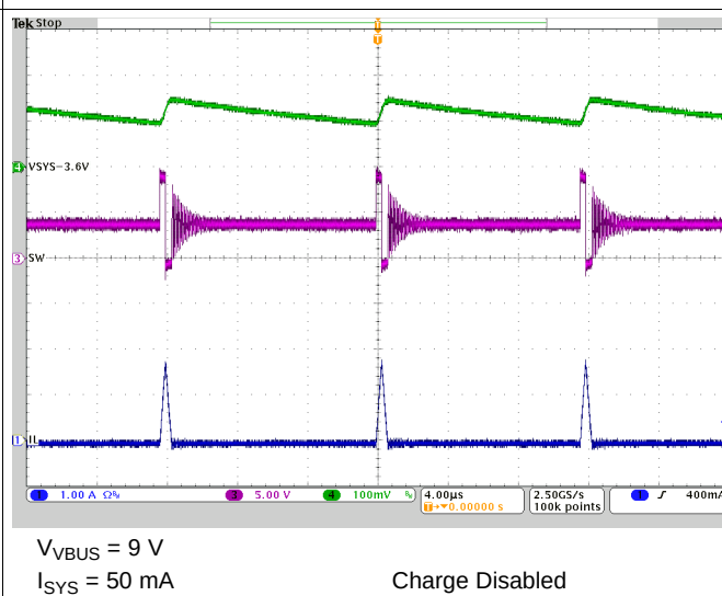
Figure 23. PFM Switching in Buck Mode
