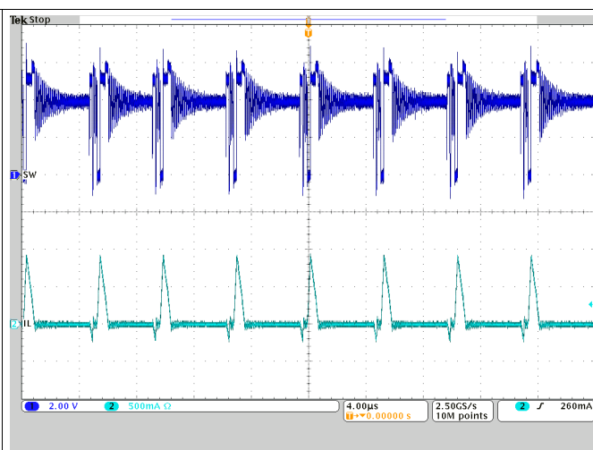
Figure 29. OTG Switching
