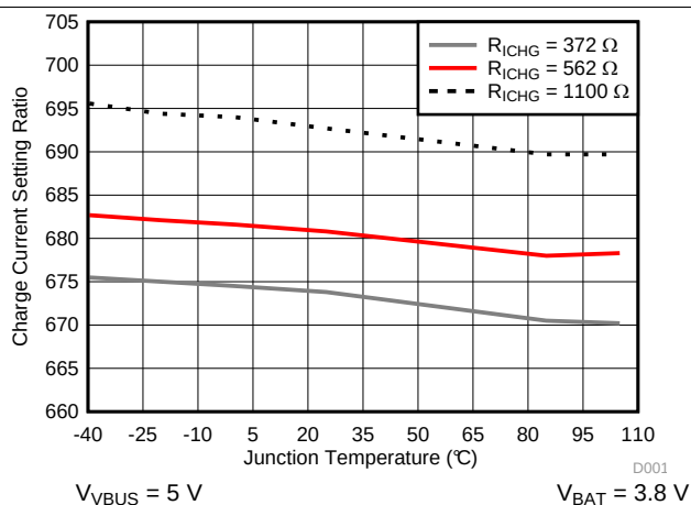
Figure 10. Charge Current Setting Ratio vs. Junction Temperature
