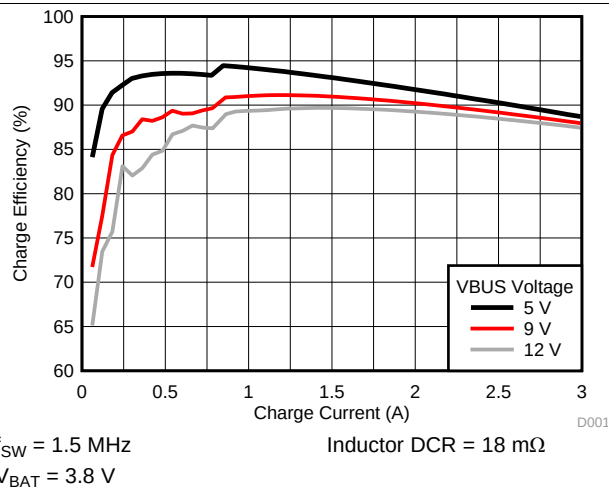
Figure 1. Charge Efficiency vs. Charge Current
