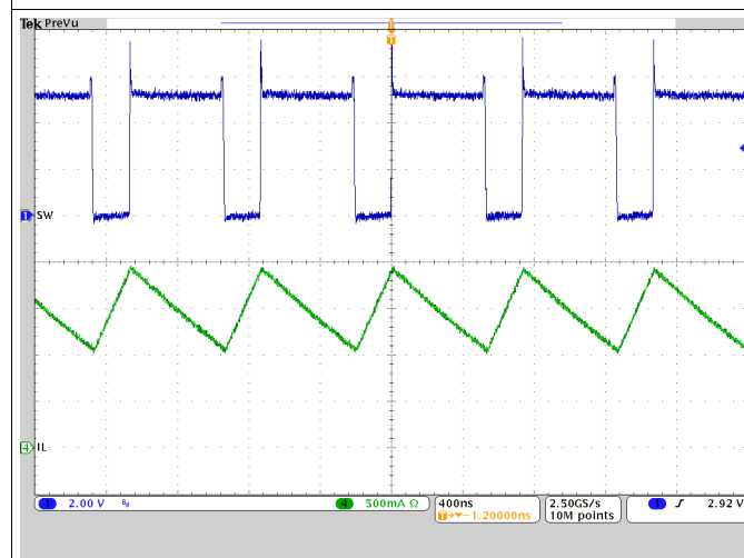
Figure 28. Charge Disable
