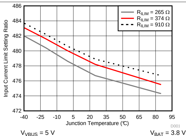
Figure 9. Input Current Limit Setting Ratio vs. Junction Temperature
