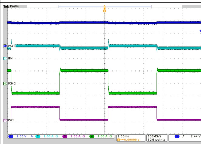
Figure 29. OTG Switching
