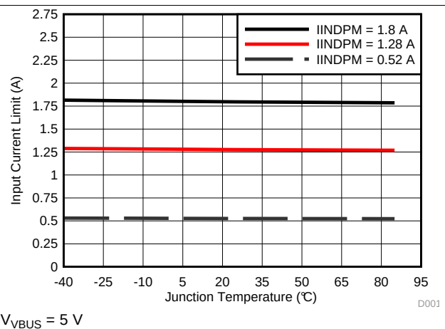
Figure 6. Input Current Limit vs. Junction Temperature
