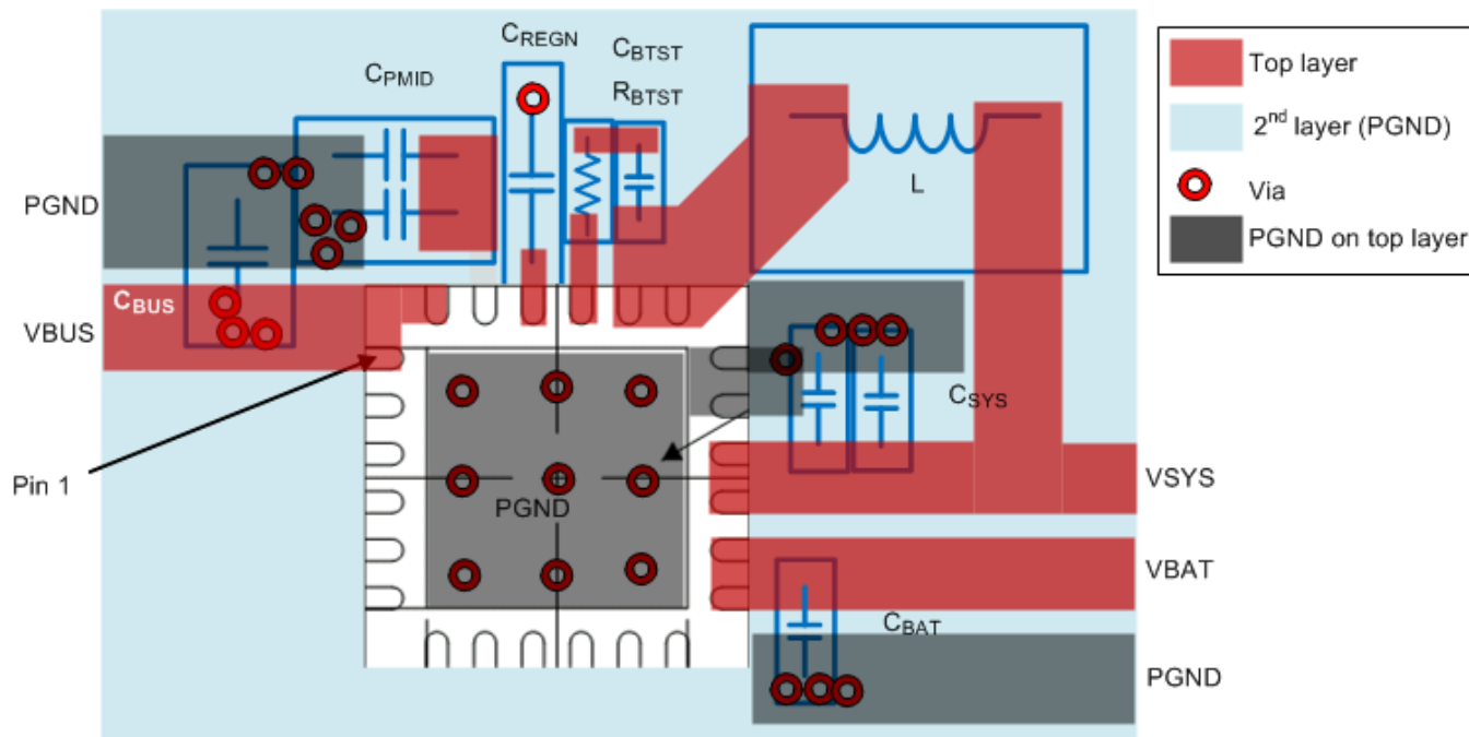
Figure 39. Layout Example
