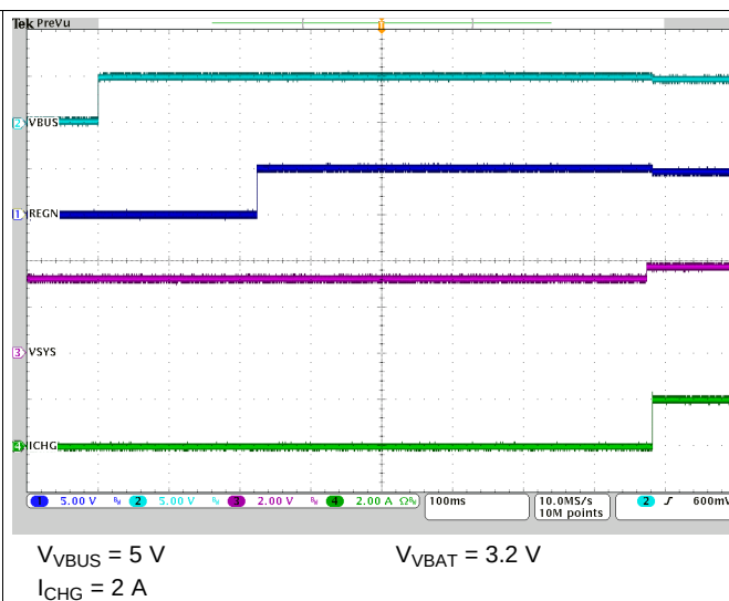
Figure 21. Power-Up with Charge Enabled
