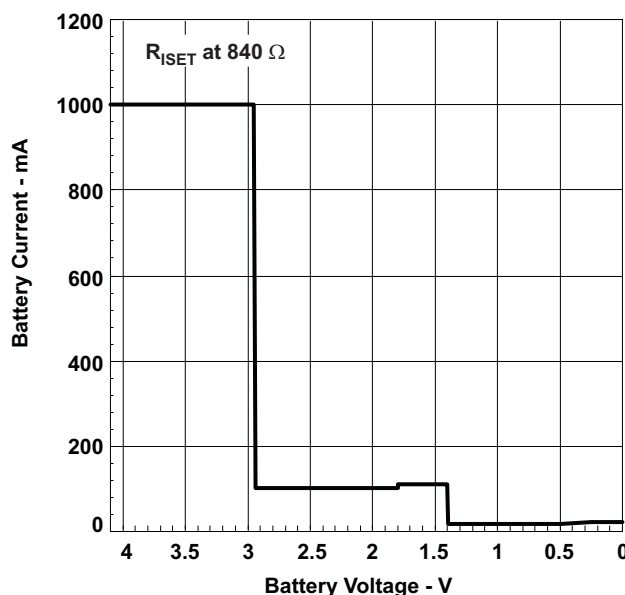
Figure 20. bq24085/6/7/8 Short Circuit Behavior
