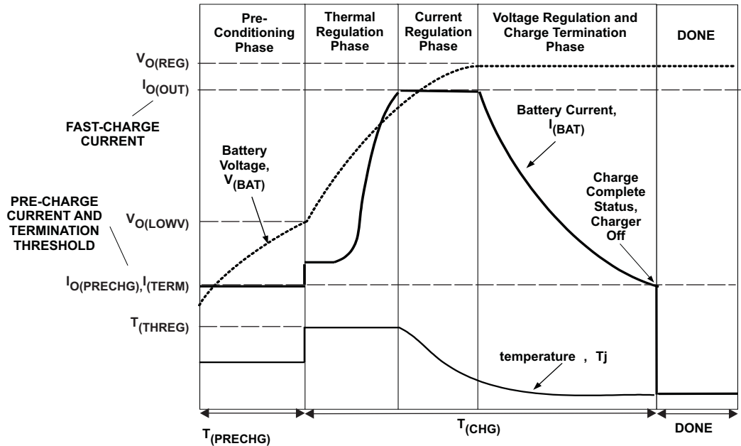
Figure 15. Charge Profile, Thermal Loop Active
