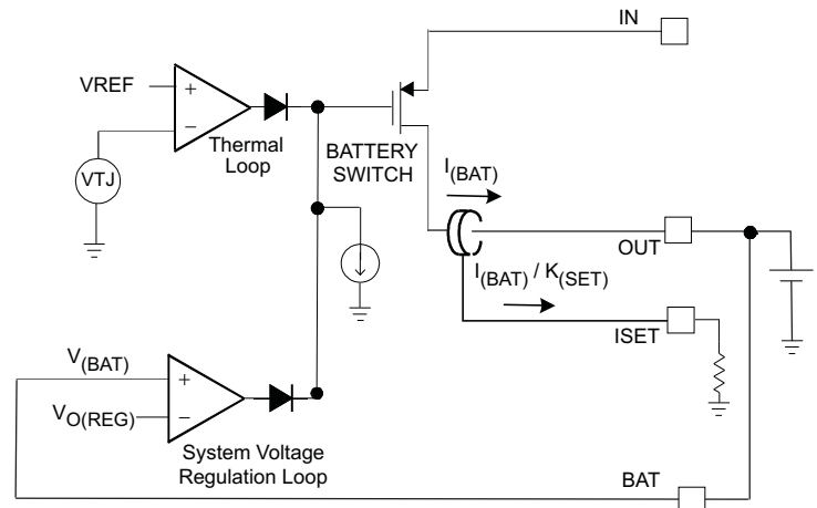
Figure 14. Thermal Regulation Circuit
