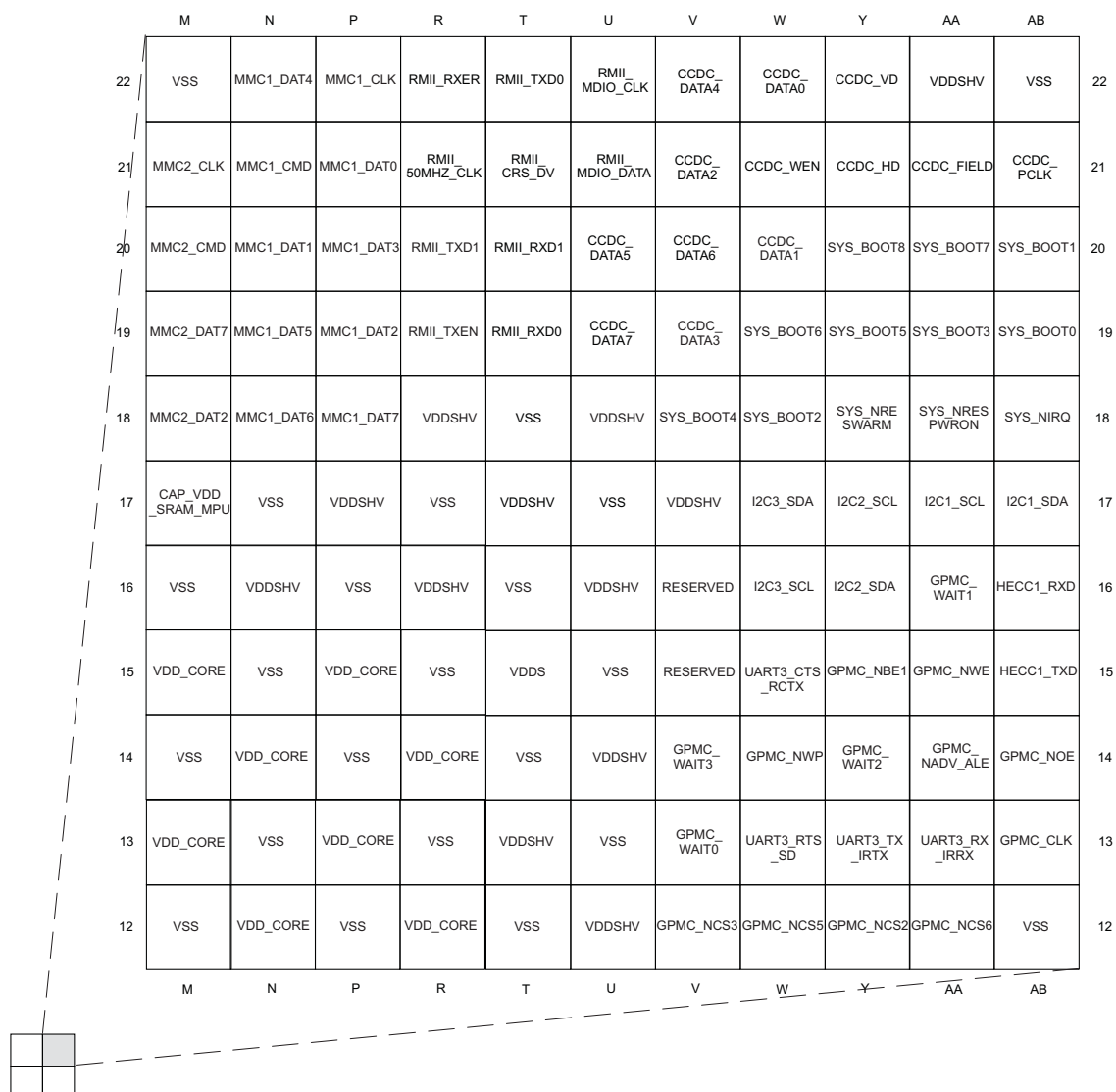
Figure 2-6. ZER Pin Map [Quadrant B]
