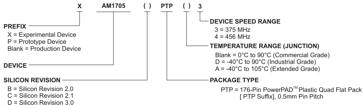
Figure 6-1. Device Nomenclature
