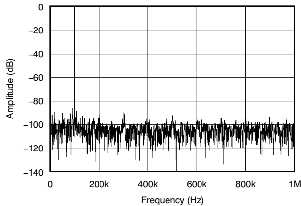
Figure 16. FREQUENCY SPECTRUM (4096-Point FFT; f_{IN} = 100 kHz)
