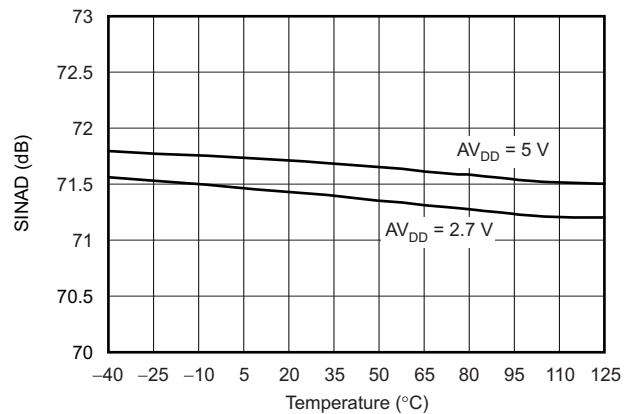
Figure 19. SIGNAL-TO-NOISE RATIO AND DISTORTION vs TEMPERATURE
