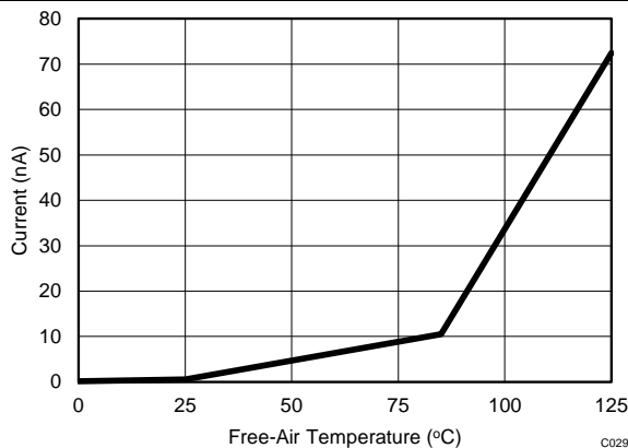
Figure 29. Supply Current vs AVDD
