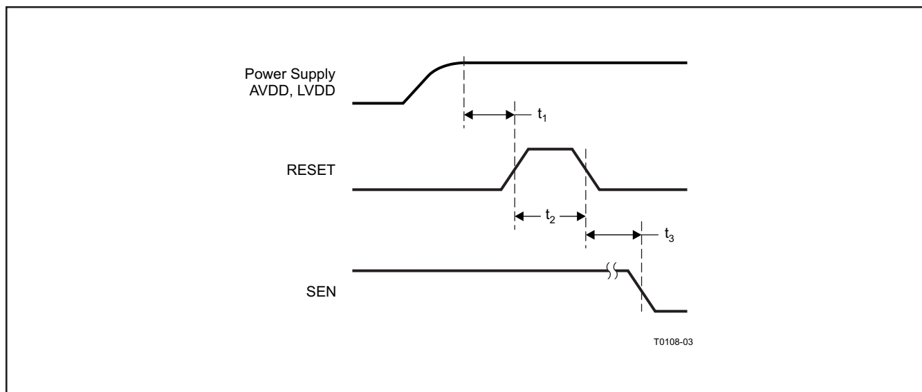
Figure 5. Reset Timing
