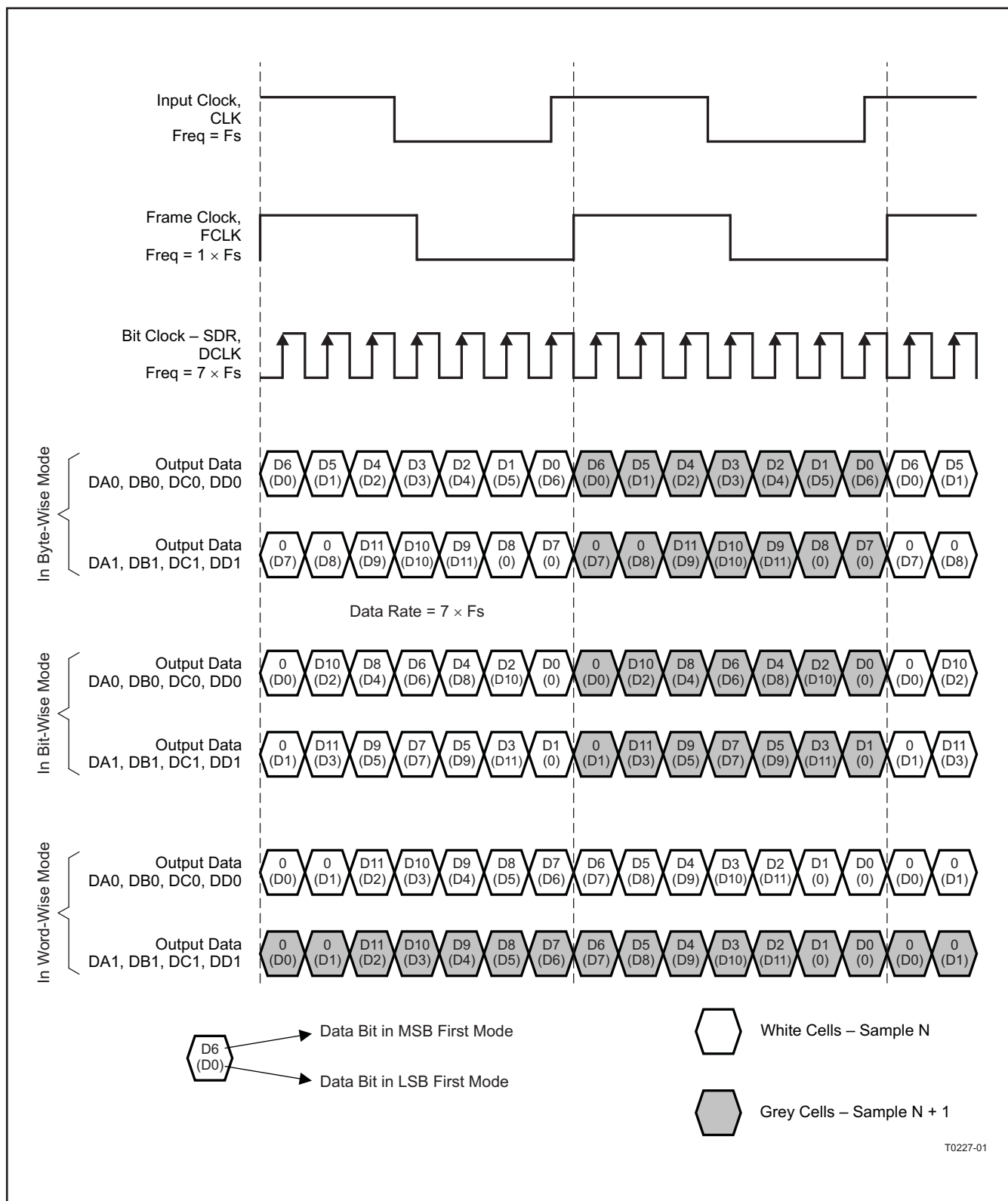
Figure 40. 2-Wire Interface 14× Serialization - SDR Bit Clock
