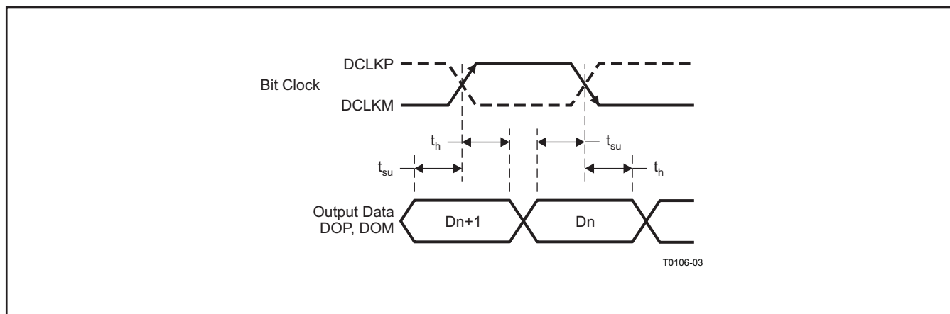
Figure 2. LVDS Timings
