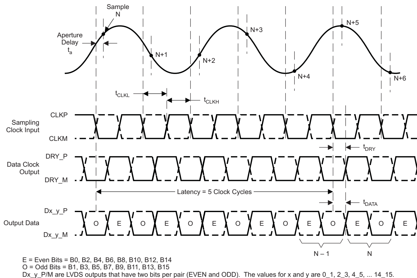
Figure 1. Timing Diagram
