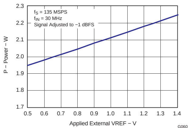
Figure 35. Total Power Consumption versus External VREF
