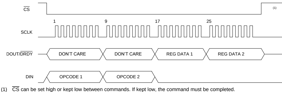
Figure 121. Read Register Sequence
