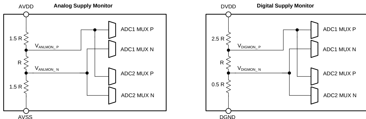
Figure 70. Power-Supply Monitors
