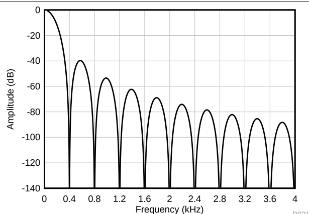
Figure 100. ADC2 400 SPS Frequency Response
