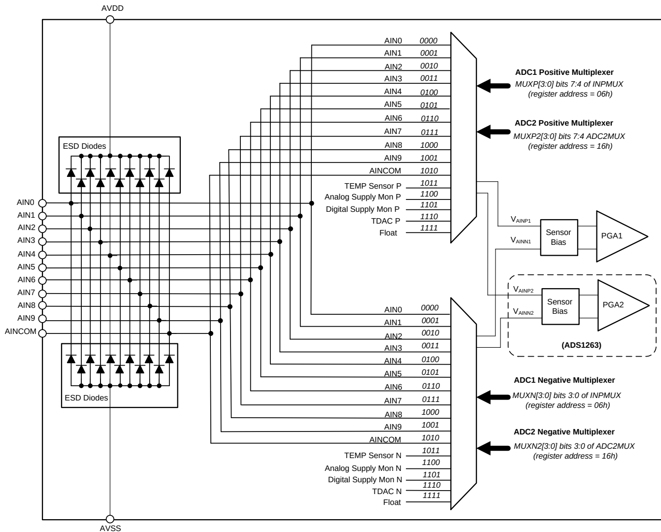
Figure 67. ADC1 and ADC2 Input Block Diagram
