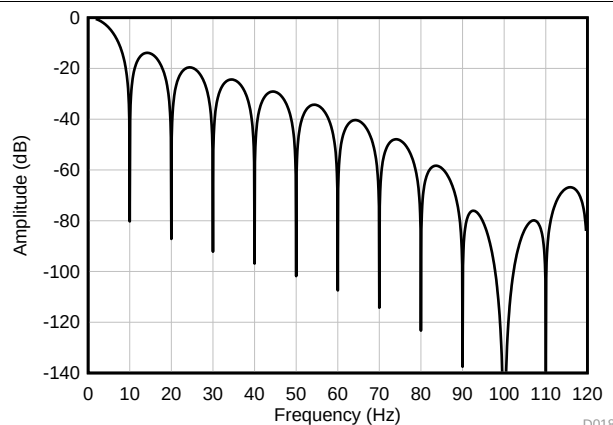
Figure 97. ADC2 10 SPS Frequency Response
