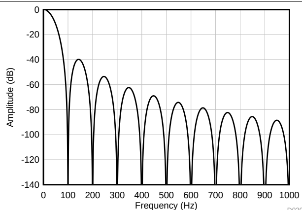
Figure 99. ADC2 100 SPS Frequency Response
