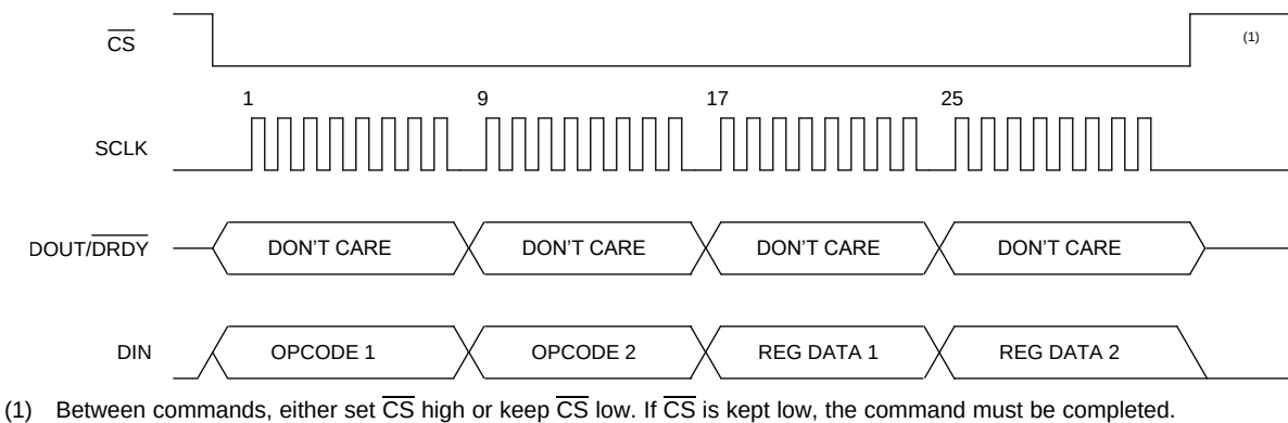
Figure 122. Write Register Sequence
