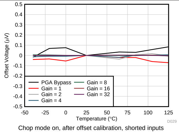
Figure 5. ADC1 Offset Voltage vs Temperature
