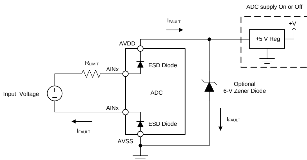
Figure 162. Analog Power-Supply Clamp
