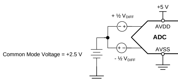
Figure 148. Differential Input with Common-Mode Level-Shift
