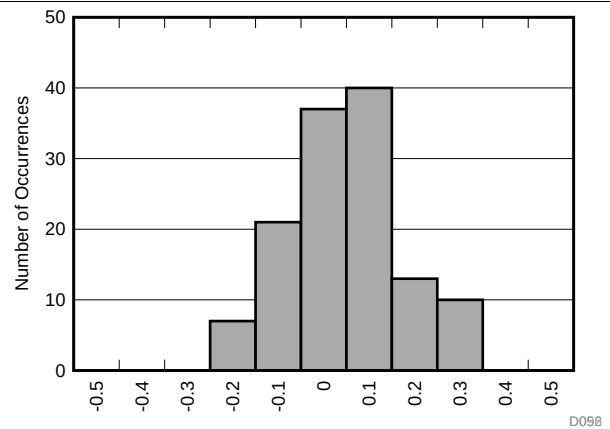
Figure 53. ADC2 Gain vs Temperature Distribution
