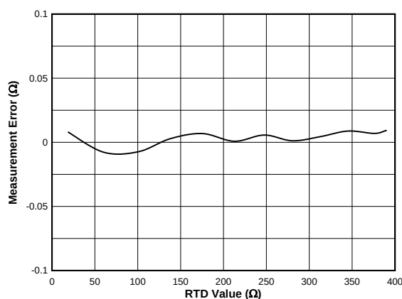
Figure 157. Resistance Measurement Error
