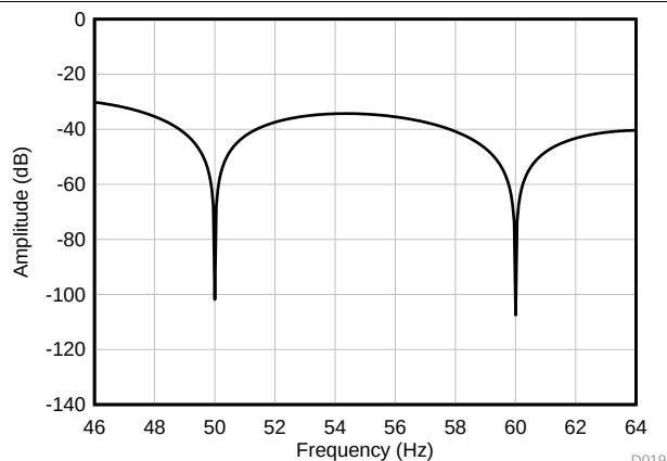
Figure 98. ADC2 10 SPS Frequency Response 50-Hz and 60-Hz Detail
