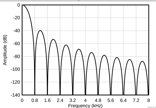
Figure 101. ADC2 800 SPS Frequency Response
