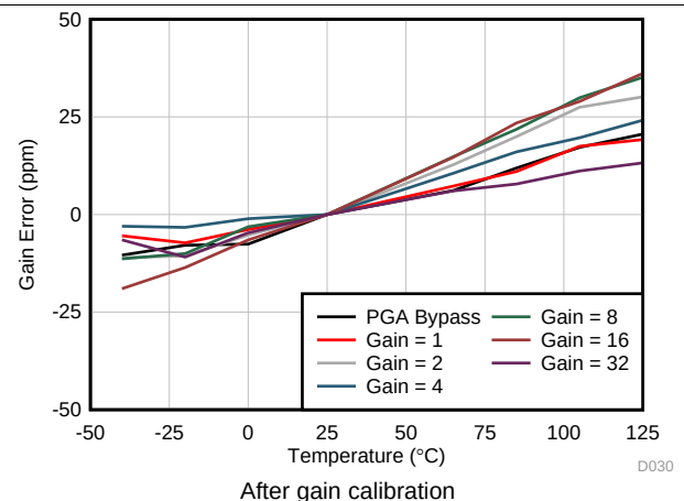
Figure 9. ADC1 Gain Error vs Temperature
