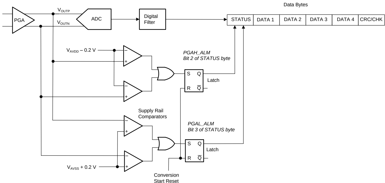
Figure 75. PGA Absolute Output-Voltage Monitor
