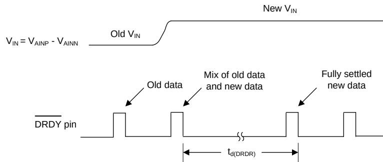
Figure 105. ADC1 Latency Timing while Continuously Converting
