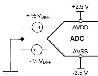
Figure 149. Differential Input with Common Mode Ground
