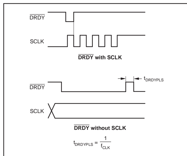
Figure 53. \overline{\text{DRDY}} Timing (See Figure 2 for the \overline{\text{DRDY}} Pulse)
