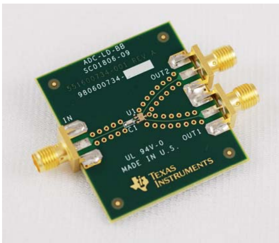
Figure 1. ADC-LD-BB
