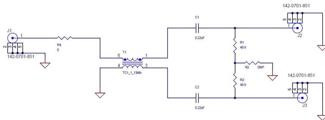
Figure 4. ADC-WB-BB Schematic
