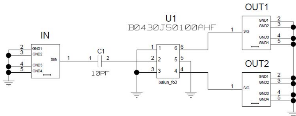
Figure 2. ADC-LD-BB Schematic
