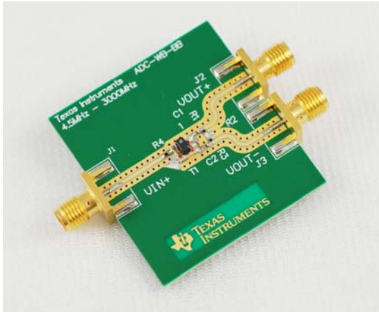
Figure 3. ADC-WB-BB
