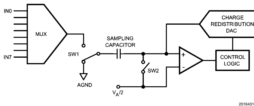
FIGURE 5. ADC108S102 in Hold Mode
