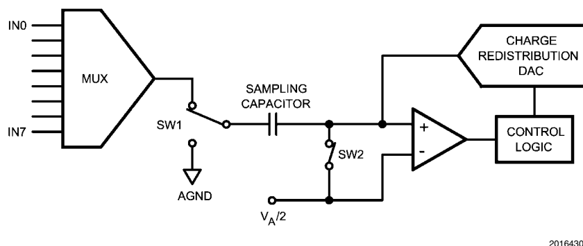
FIGURE 4. ADC108S102 in Track Mode
