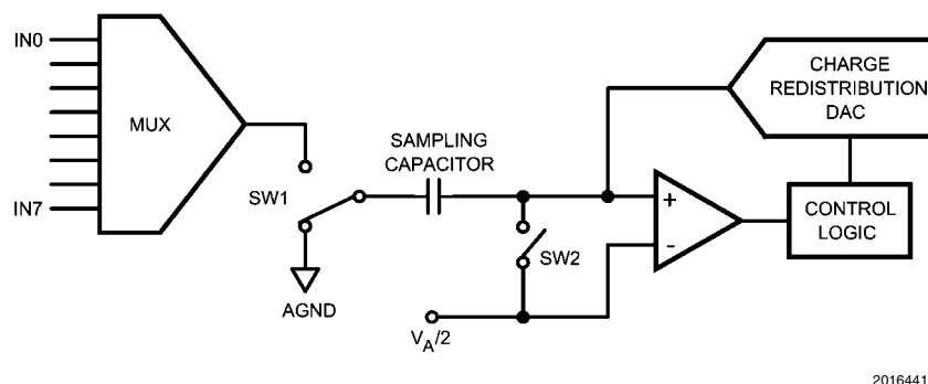
FIGURE 5. ADC108S052 in Hold Mode
