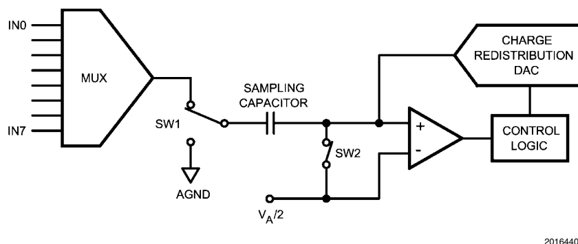
FIGURE 4. ADC108S052 in Track Mode
