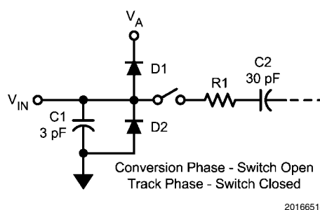
FIGURE 7. Equivalent Input Circuit
