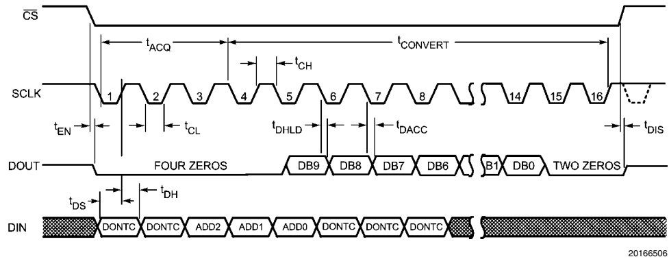
FIGURE 2. ADC088S102 Serial Timing Diagram
