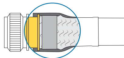
Backshell with pre-installed braid tail and heatshrink boot. Installed on cable with heat gun. Used on: KTKK/TAK
