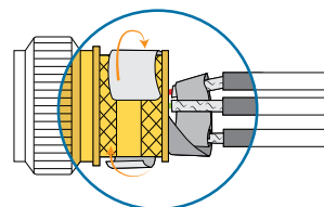
Wraps mesh tape wraps around individual screens to eliminate EMC windows Used on: KMA Series
