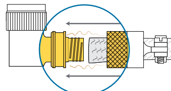
Braid trapped in loose fitting thread Used on: 95/77 Series
