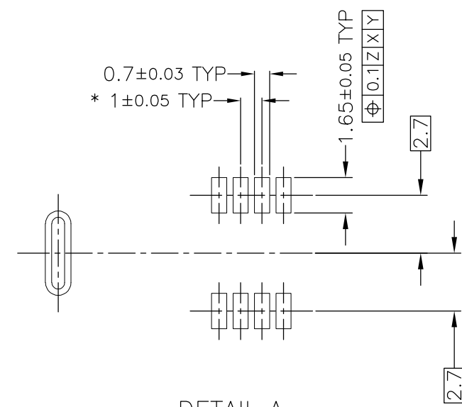
DETAIL A (4:1)
