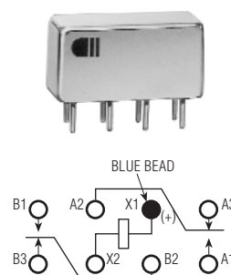
TERMINAL VIEW
