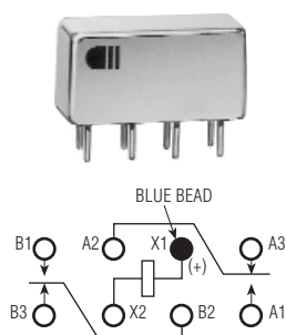
TERMINAL VIEW
