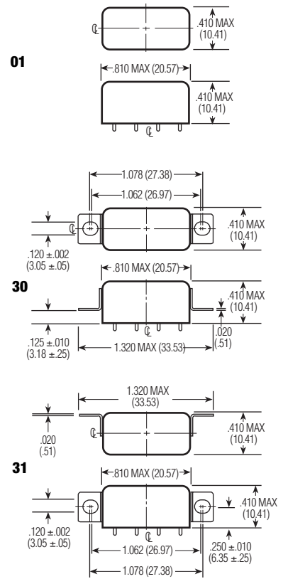
MOUNTING STYLES
