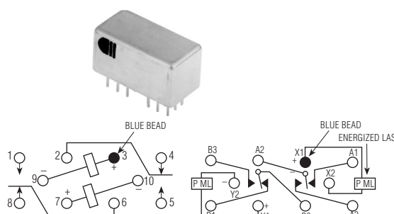
TERMINAL VIEW
