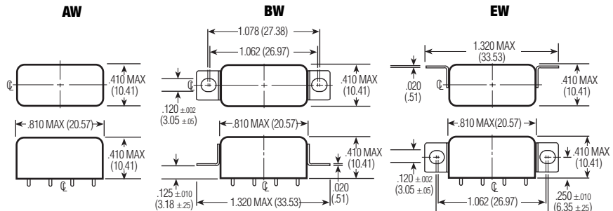
MOUNTING STYLES
