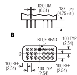
LR TERMINALS
