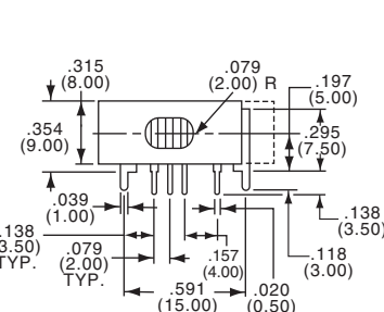
SP3T/DP3T
