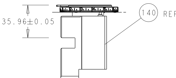
RAM SET-UP
